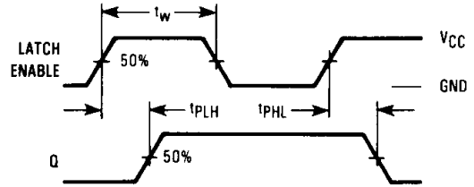
Figure 2. Switching Waveforms
