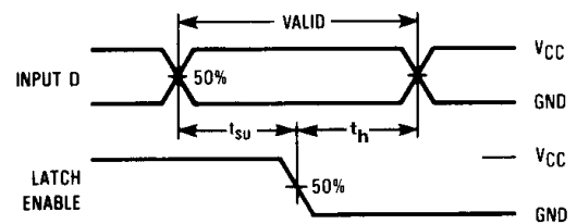
Figure 4. Switching Waveforms
