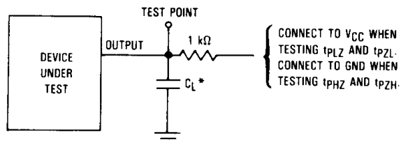
Figure 6. Test Circuit
